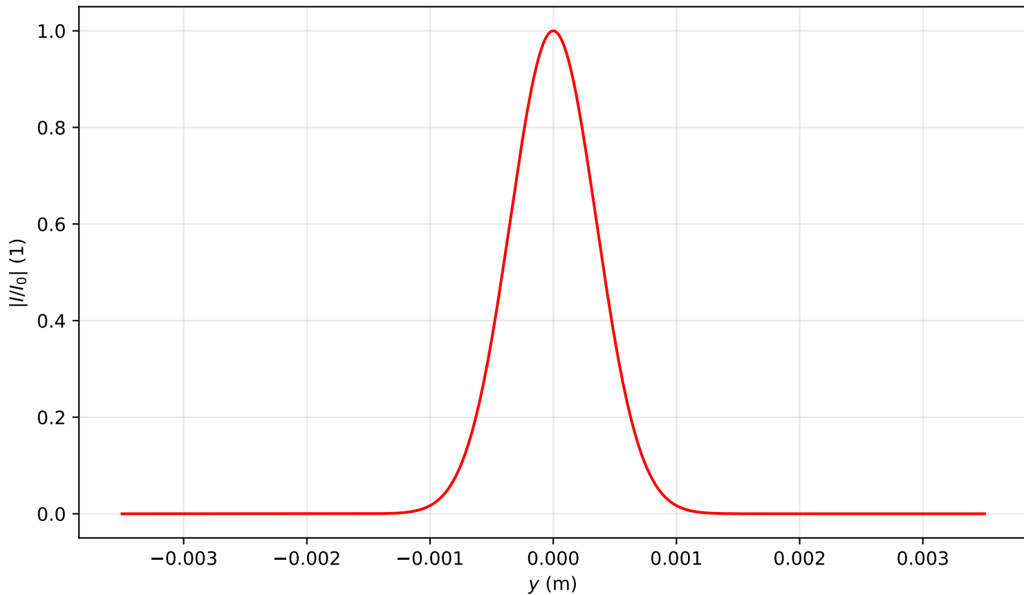
Intensity profile I(x=0, y, z=0.000)/I_0 , P_{in}=1.0P_{cr} , artificial time
